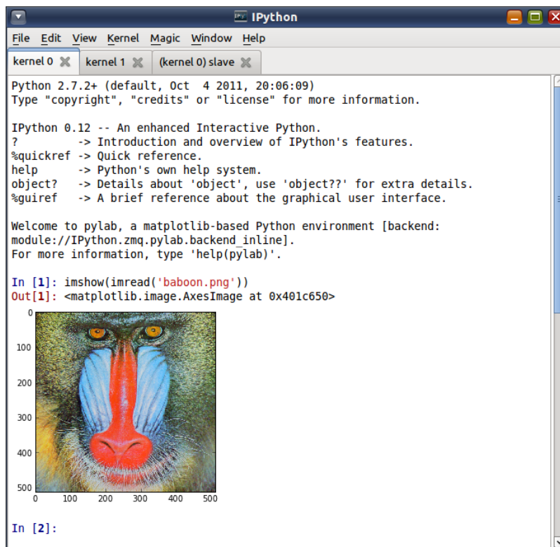
Рис. 4: The improved Qt console for IPython, now with tabs to control multiple kernels and full menu support.
